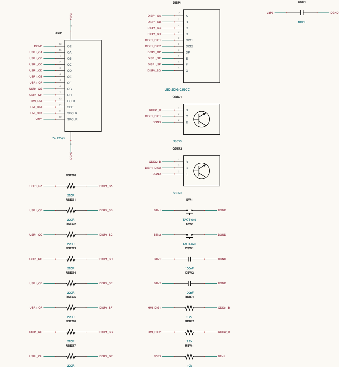
CONTROL / INTERCONNECT
