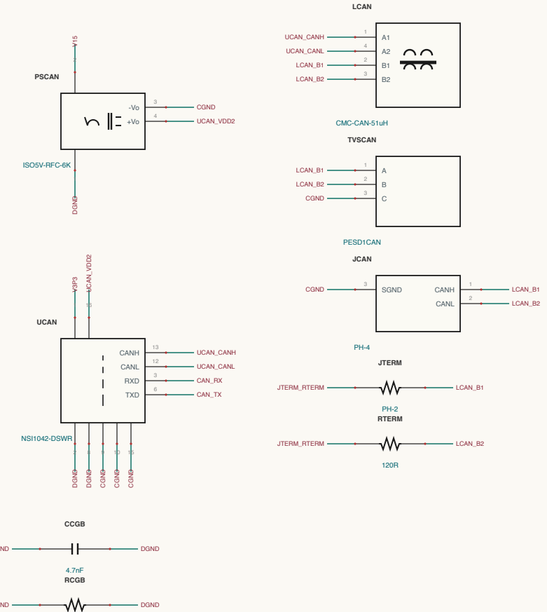
LLC-LESS / BUS-IN
